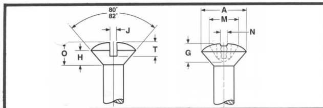
SLOTTED PHILLIPS
