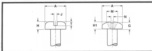
SLOTTED PHILLIPS
