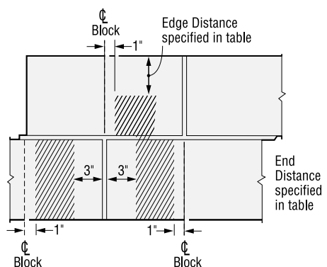
Allowable Anchor Placement in grout filled CMU shown by shaded areas.
